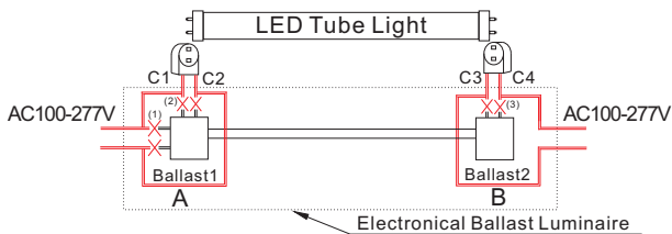
D. The luminaire with electronical ballast
