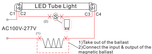
C. The Luminaire with magnetic ballast & starter
